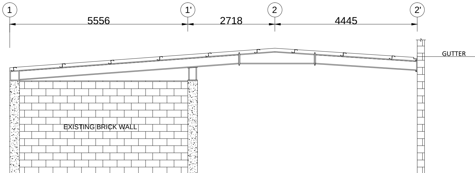
CROSS SECTION GRID-C
